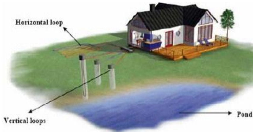
Fig. 1. Using the soil, bedrock or groundwater as the heat source.
