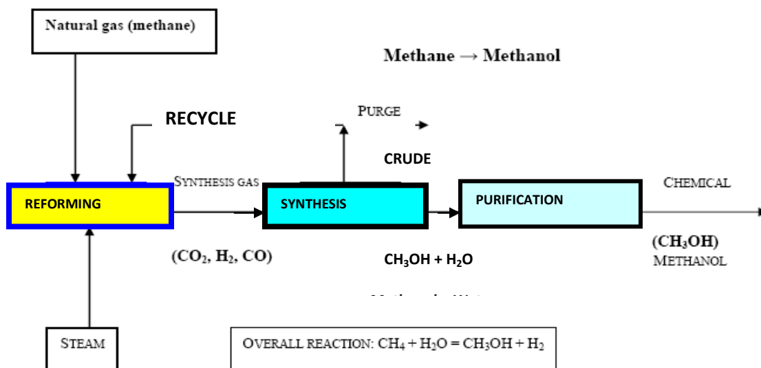
Fig. 2. Schematic diagram shows methanol production (Omer, 2006).
