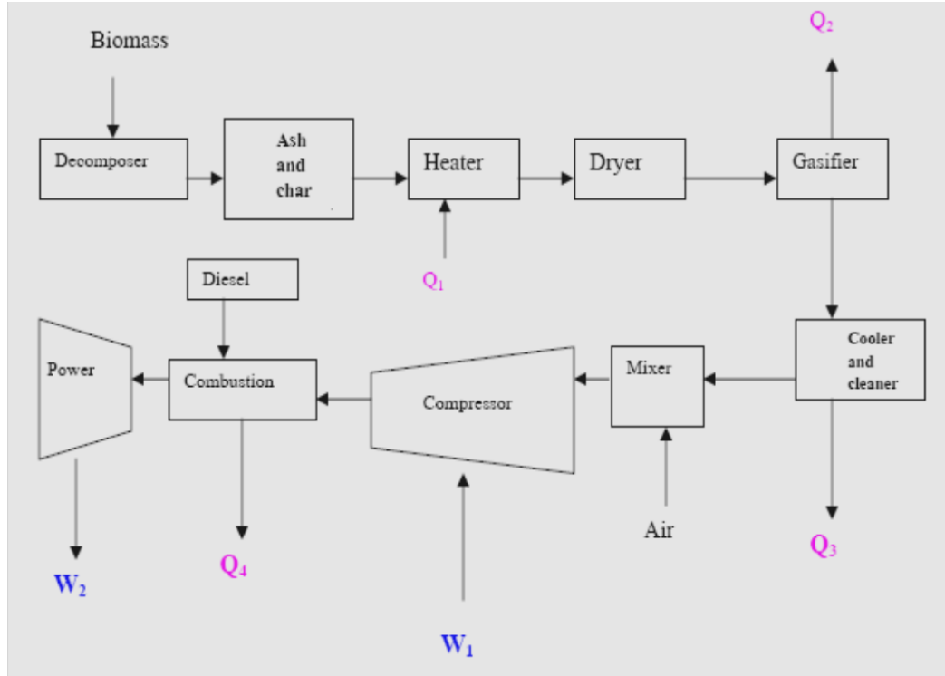
Fig. 7. Advanced biomass power with diesel engine (Omer, 2006).
