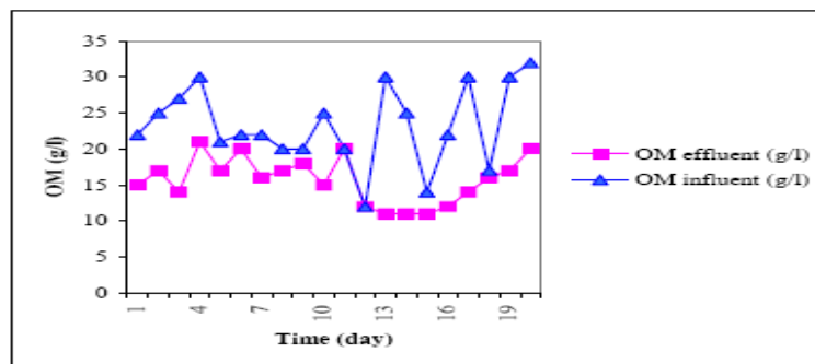
Fig. 5. Organic matters before and after treatment in digester (Omer, 2006).
