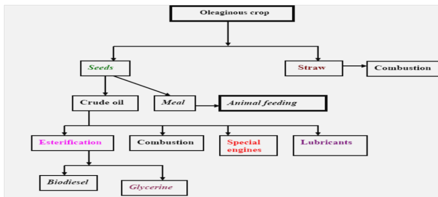
Fig. 9. Flow chart of biodiesel production (Omer, 2006).
