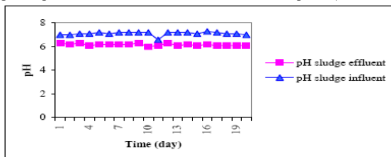
Fig. 6. pH sludge before and after treatment in the digester (Omer, 2006).
