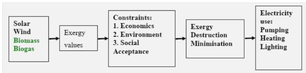
Fig. 11. Exergy based optimal energy model (Omer, 2008).
