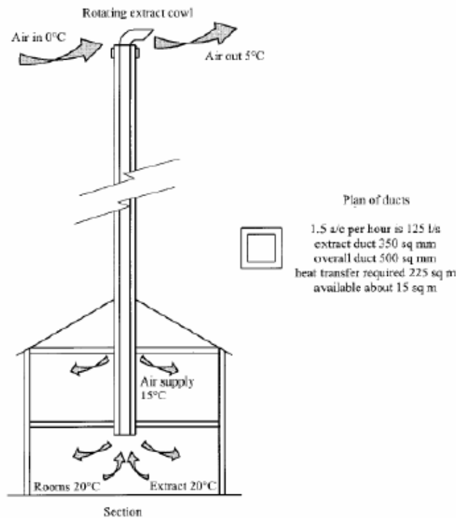
Fig. 2. Small house natural ventilation with heat reclaims (A very tall chimney) (Fordham, 2000).
