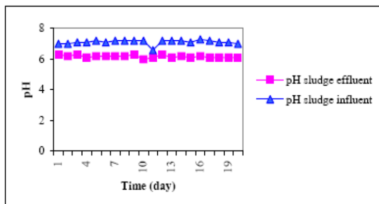
Fig. 6. pH sludge before and after treatment in the digester (Omer, 2006).
