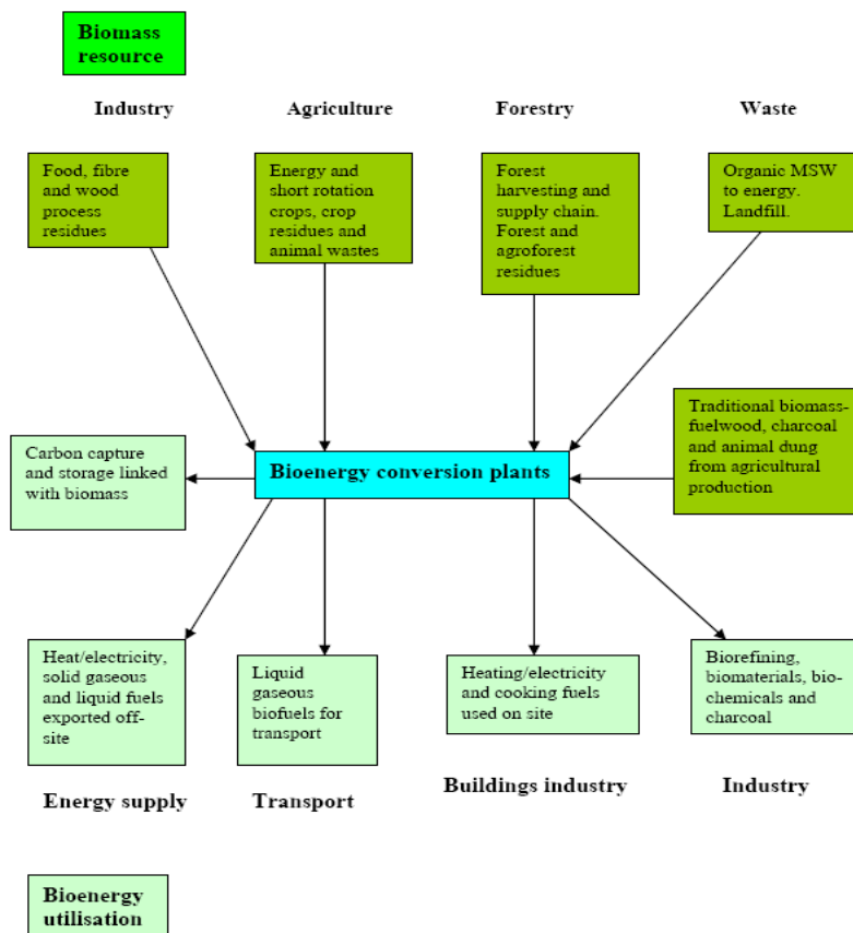
Fig. 4. Biomass resources from several sources are converted into a range of products for use by transport, industry and building sectors (Sims, 2007).
