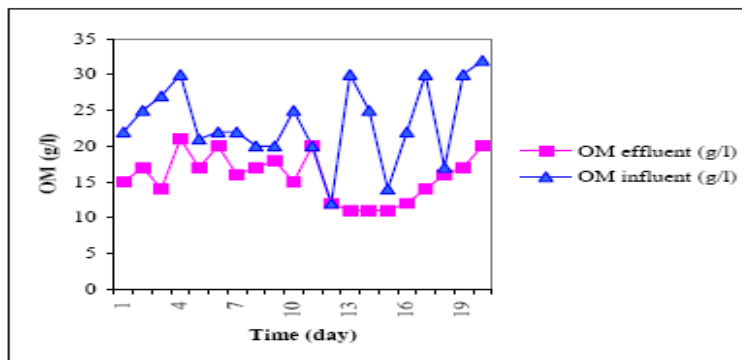
Fig. 5. Organic matters before and after treatment in digester (Omer, 2006).
