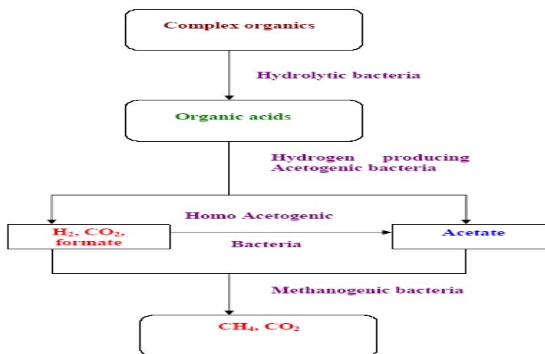
Fig. 3. Biogas production process (Omer, 2003).
