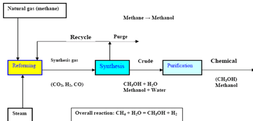
Fig. 2. Schematic diagram shows methanol production (Omer, 2006).
