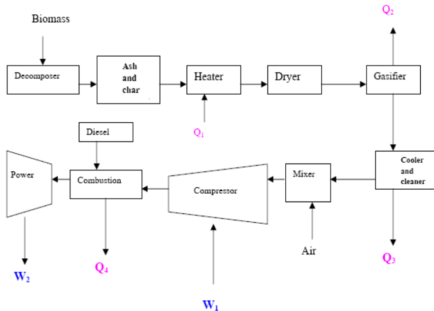
Fig. 7. Advanced biomass power with diesel engine (Omer, 2006).
