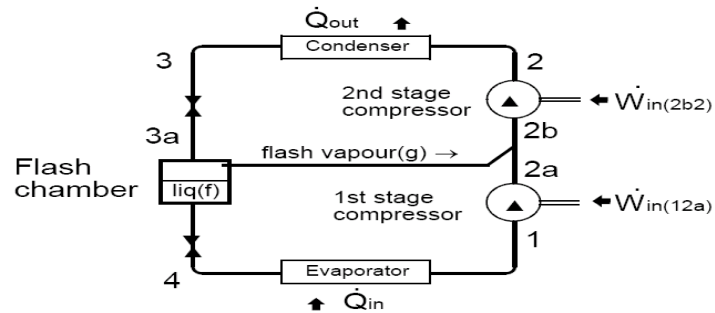
Fig. 20. Liquid-suction heat exchanger cycle.
