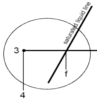
Fig. 17. Condenser sub-cooling.
