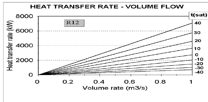
Fig. 5. Heat transfer rate versus volume rate.
