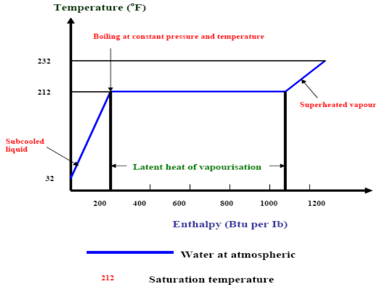
Fig. 13. Water undergoing a change of state.
