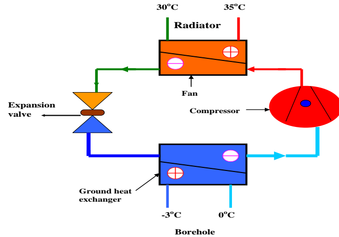
Fig. 2. Detail of the GSHP circuit.
