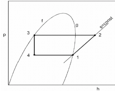
Fig. 14. Refrigeration cycle.
