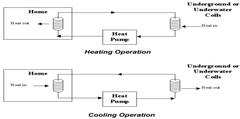
Fig. 10. Heating and cooling operations.
