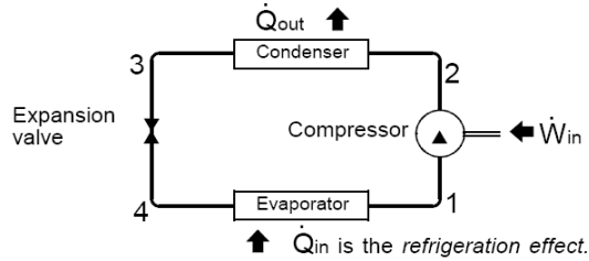
Fig. 7. Simplified refrigeration system diagram.
