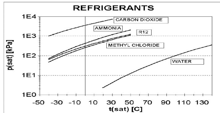
Fig. 9. Refrigerant chart.
