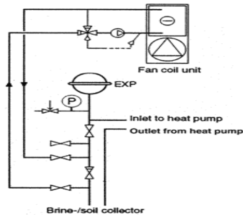
Fig. 3. Diagram of cooling system.
