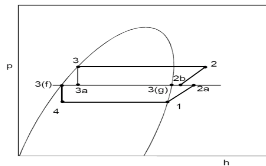
Fig. 21. Cycle of multiple compressions using flash chamber.
