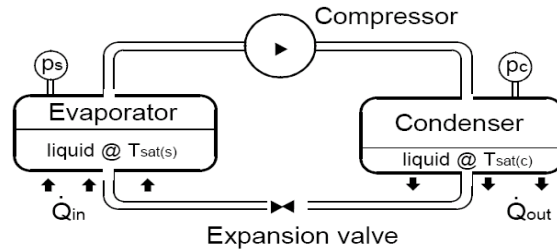
Fig. 8. Heat pump refrigeration cycle.
