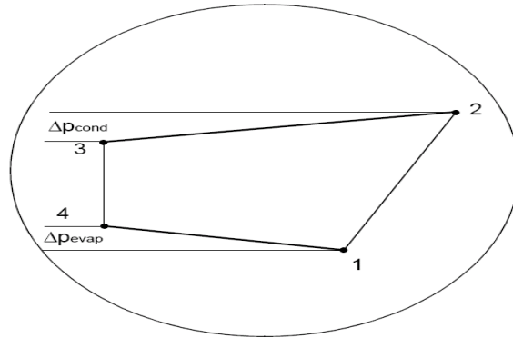
Fig. 18. Pressure drops in evaporator and condenser.
