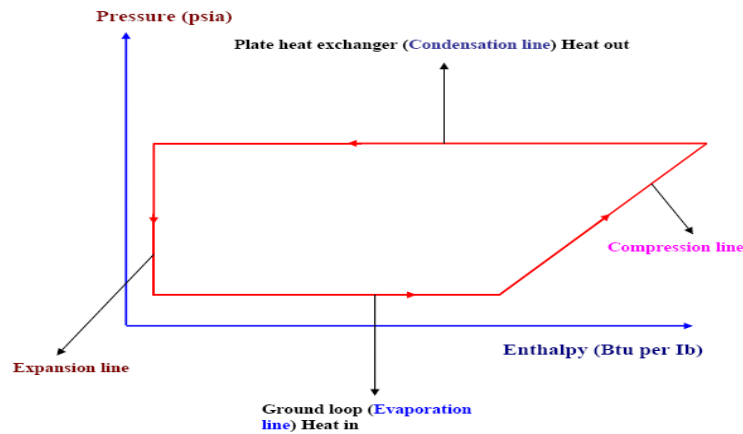
Fig. 12. The ideal cycle on Pressure-Enthalpy diagram.
