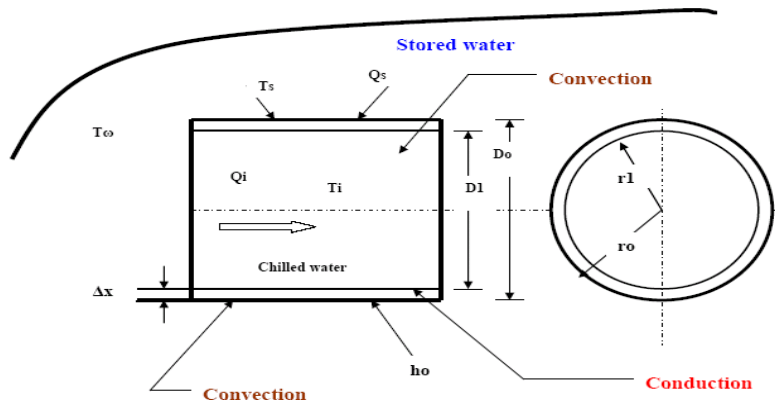
Fig. 11. Schematic of heat transfer through a circular tube heat exchanger.
