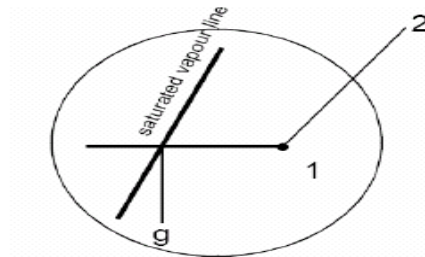
Fig. 15. Evaporator superheat.
