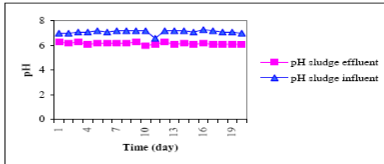
Fig. 6. Potential of hydrogen (pH) sludge before and after treatment in the digester.
