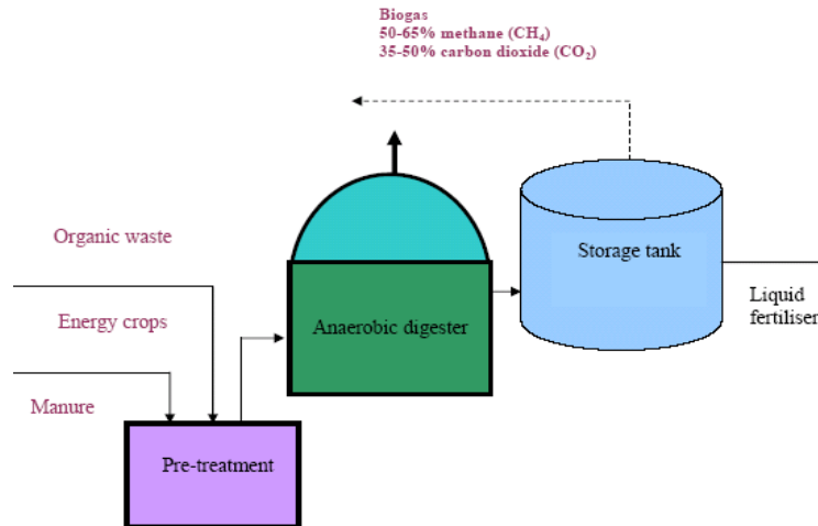
Fig. 1. General schematic of an agricultural biogas plant (Abdeen, 2012).
