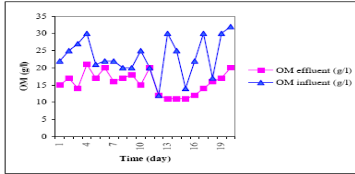
Fig. 5. Organic matters before and after treatment in digester.
