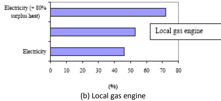
Fig. 2. Greenhouse gas emissions savings for different biogas utilisation pathways in comparison to fossil energy production.
