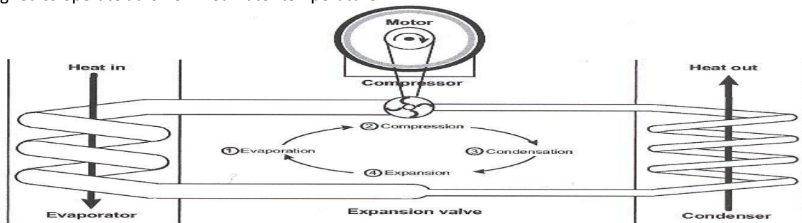
Fig. 4. Ground source heat pumps.
