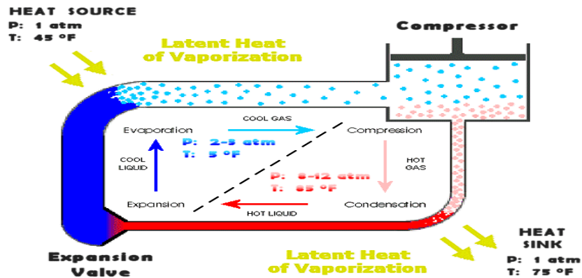
Fig. 6. Heat pump works by promoting the evaporation and condensation of a refrigerant.
