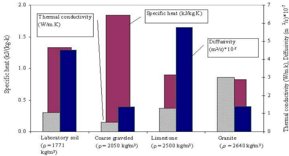
Fig. 1. Measured thermal properties for different soils.
