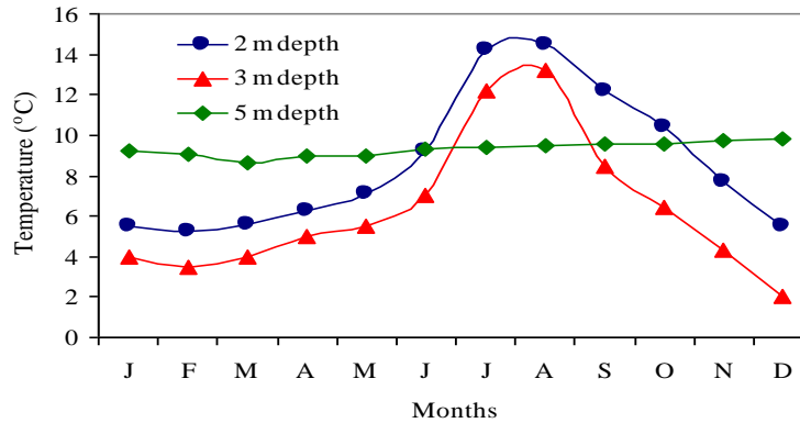
Fig. 7. Ground temperatures throughout the year.
